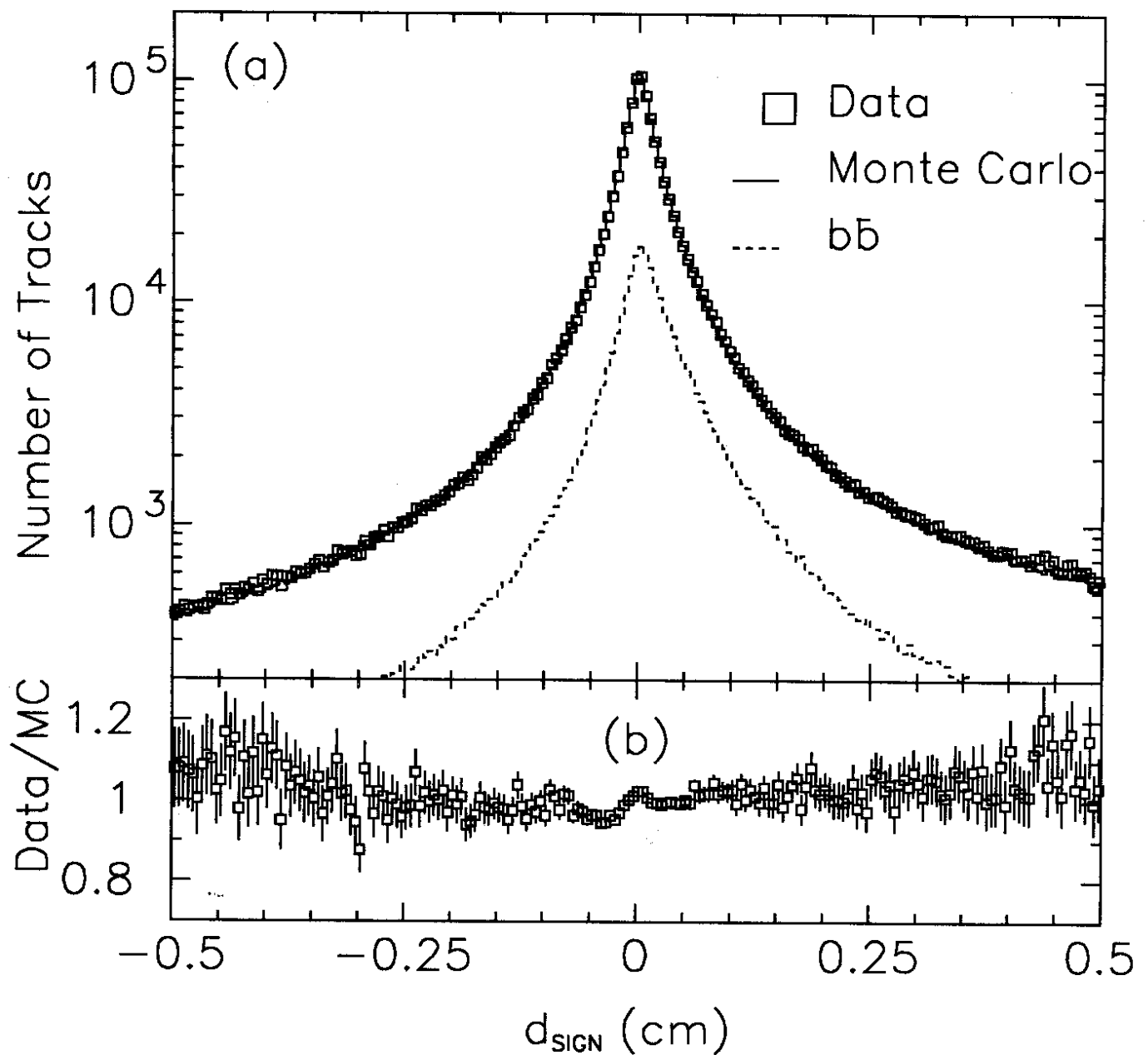
Figure 3: The distribution of the signed impact parameter for all the data tracks (squares) that meet the selection criteria. The solid line shows the same distribution for the Monte Carlo. The dashed line shows the Z^0 \rightarrow b\bar{b} component of the Monte Carlo distribution. The ratio of the data to the Monte Carlo is shown in (b).
